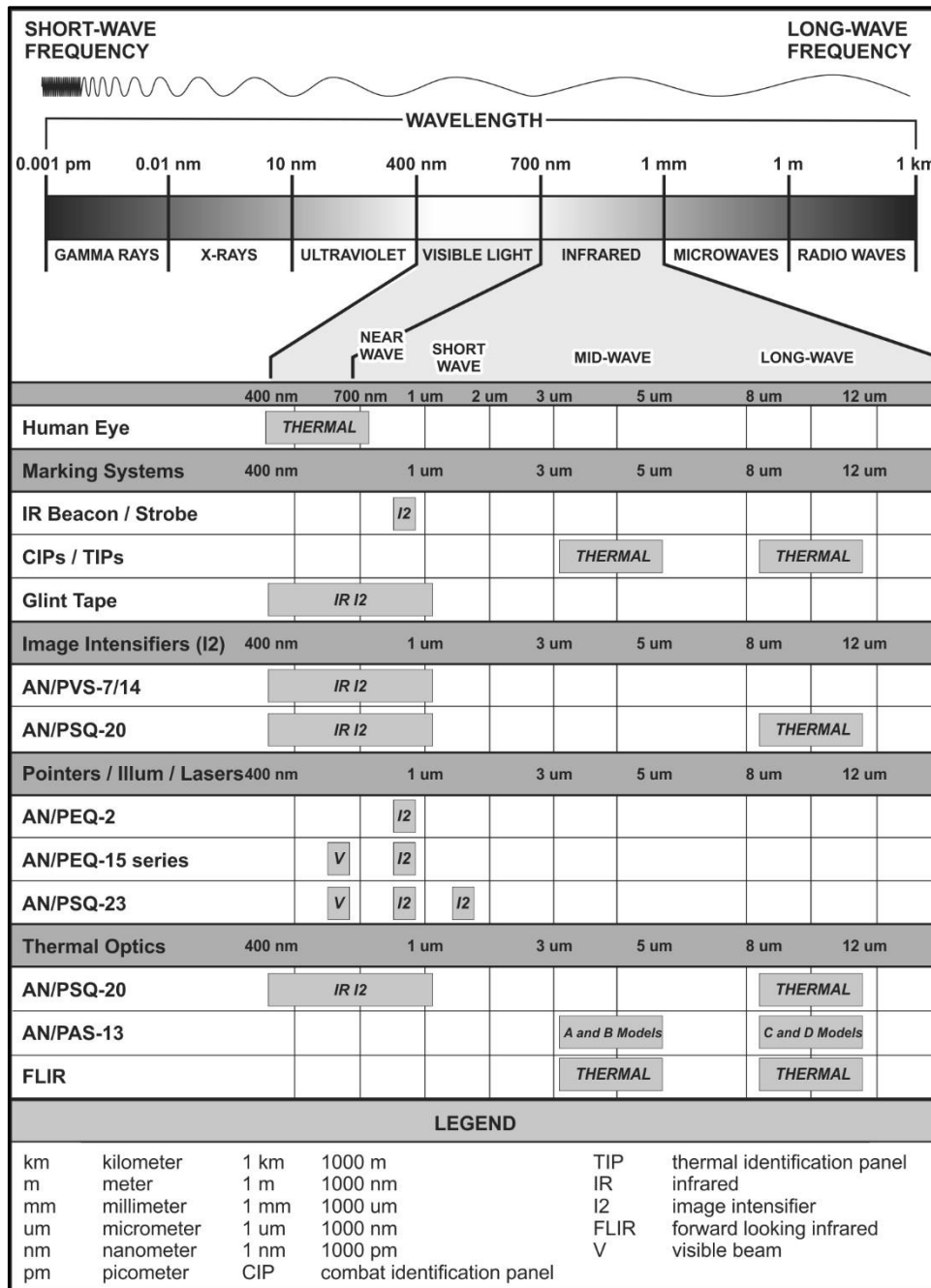
Figure 3-5. Electromagnetic spectrum
